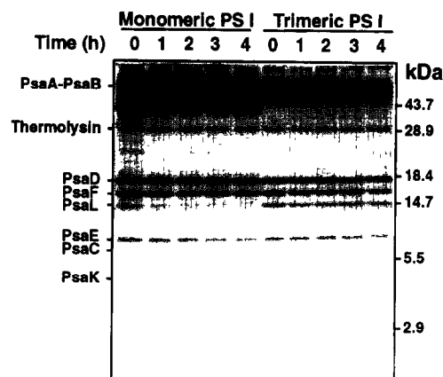
Fig. 3. Protease accessibility of PSI subunits in monomeric and trimeric complexes. The monomers and trimers of PSI were diluted to 100 \mu g chlorophyll/ml and incubated with thermolysin (50 \mu g/mg chlorophyll) and 1 mM \text{CaCl}_2 for 0, 1, 2, 3, 4 h. Subsequently, the reactions were terminated by addition of 25 mM EDTA and the proteins were solubilized by incubating samples with 1% SDS and 0.1% \beta -mercaptoethanol for 1 h at room temperature and were separated using Tricine-urea-SDS-PAGE. The proteins were stained with Coomassie blue. The experiment was repeated six times, using different periods of proteolysis. Polypeptide profiles of PSI after proteolysis in a representative experiment are shown.
